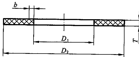
(c) RF-E型
